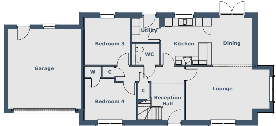
Ground Floor
